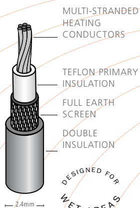
wire cross-section
