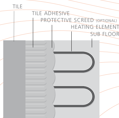
installation diagram
